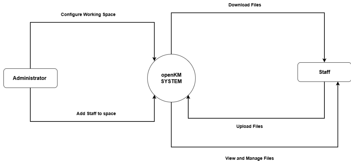
Figure 2.8: OpenKM context diagram
