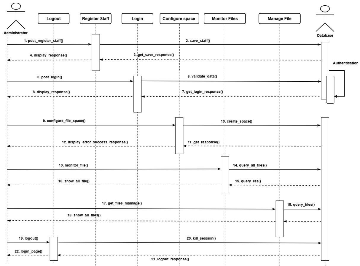
Figure 2.10: OpenKM sequence diagram
