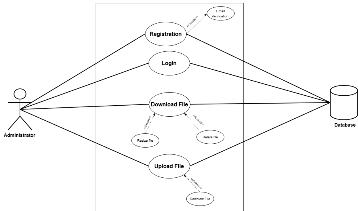
Figure 2.6: File stack use case diagram
