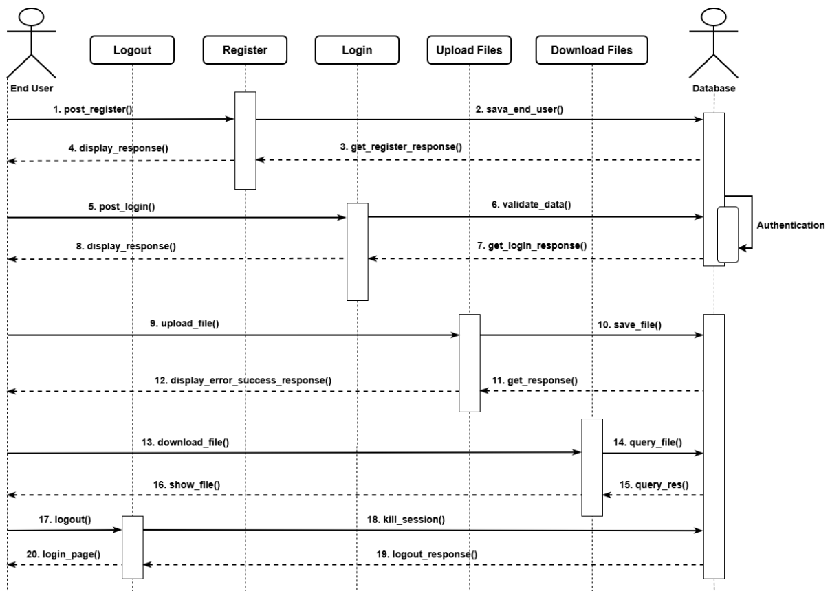
Figure 2.3: Upload care sequence diagram for user
