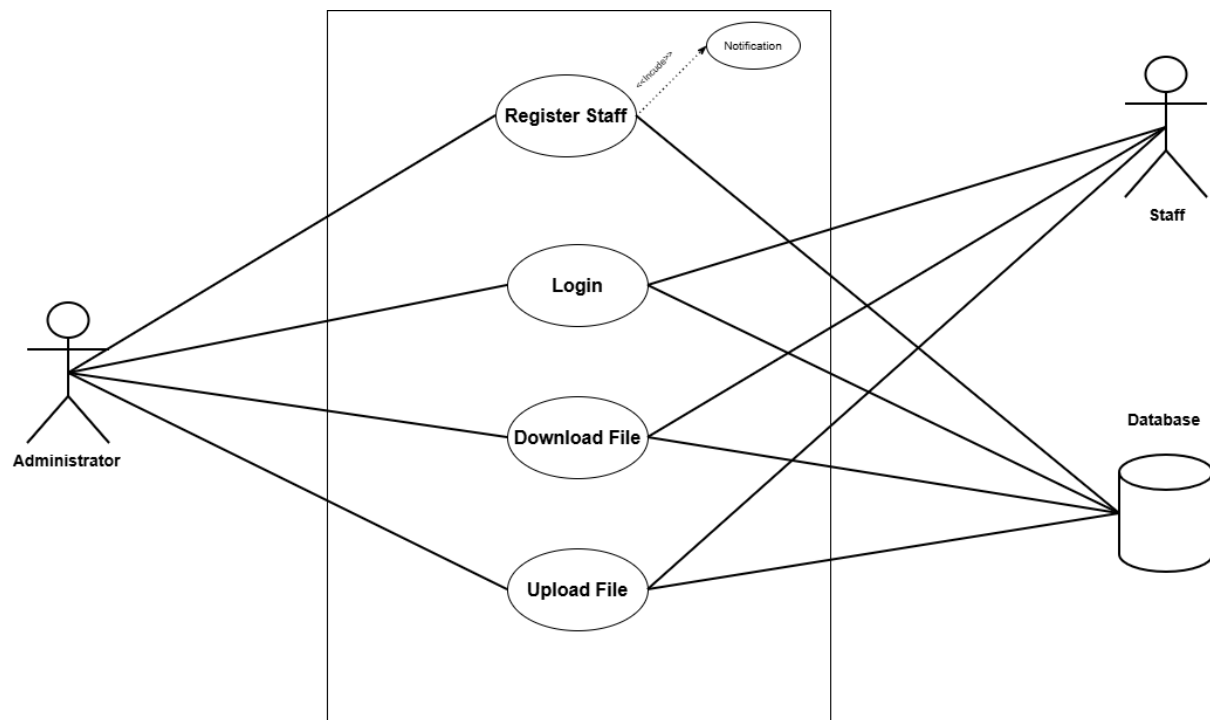
Figure 2.9: OpenKM use case diagram
