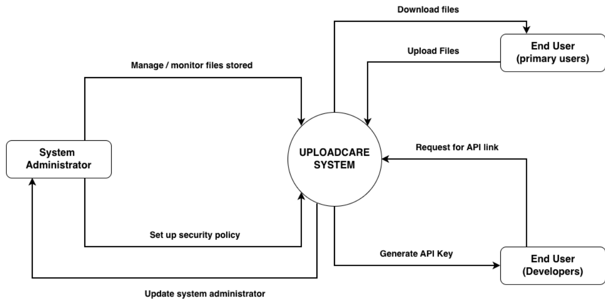
Figure 2.1: Upload care context diagram
